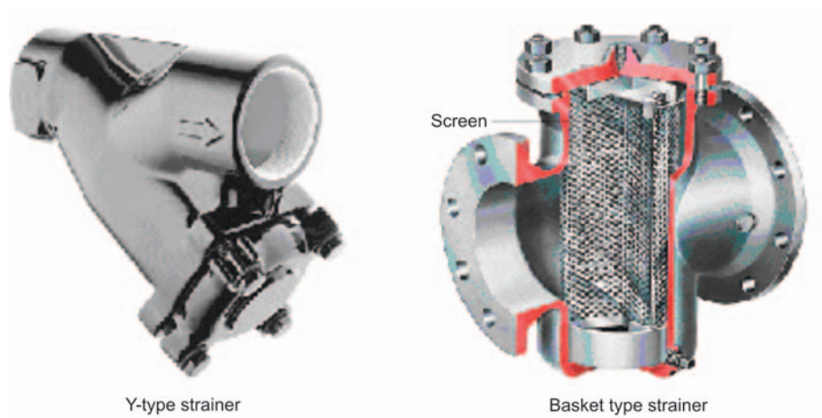
Figure 3.14 Strainers
