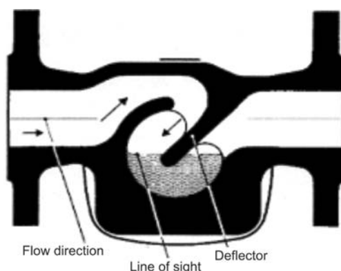
Figure 3.15 Sight Glass
