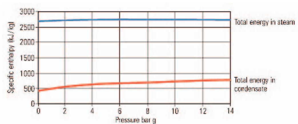
Figure 3.23 Heat Content of Steam and Condensate at the Same Pressure
