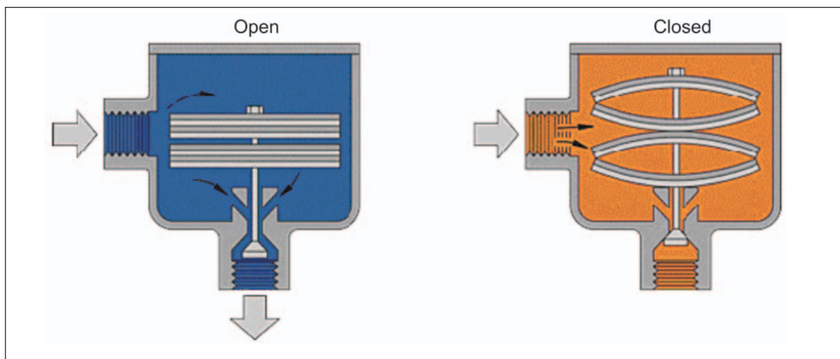
Figure 3.9 Bimetallic Type
